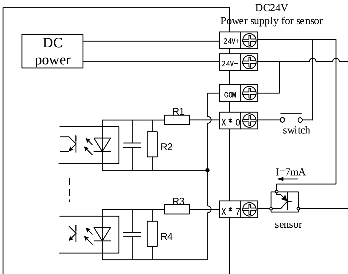
PNP type
