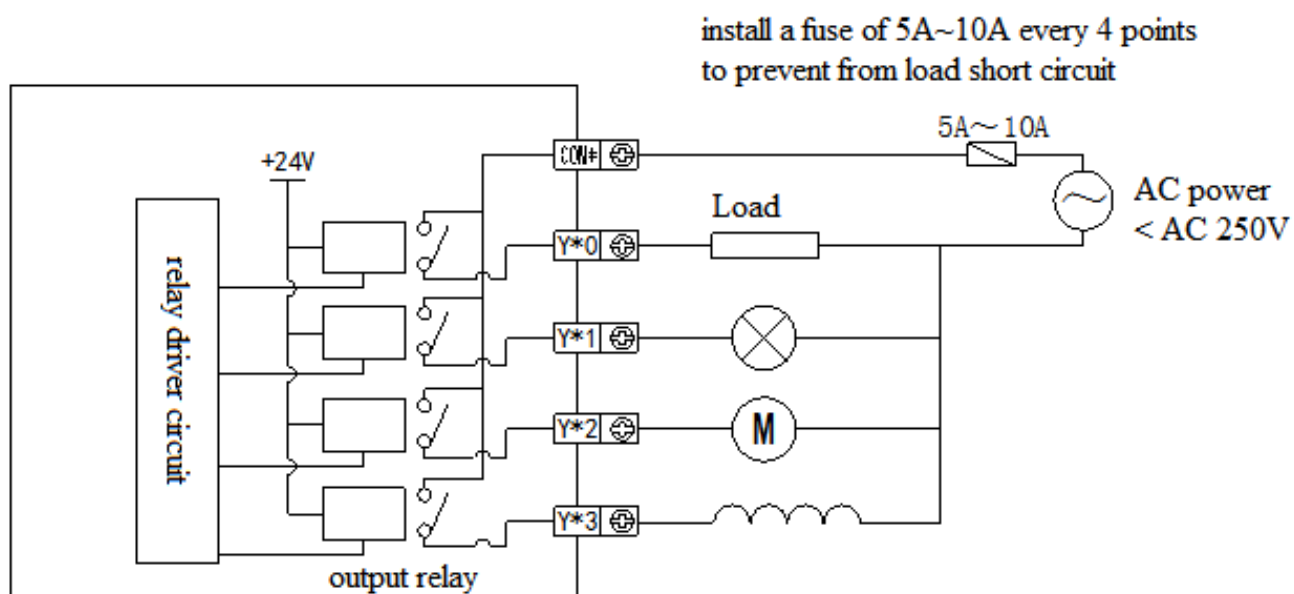
Relay type
