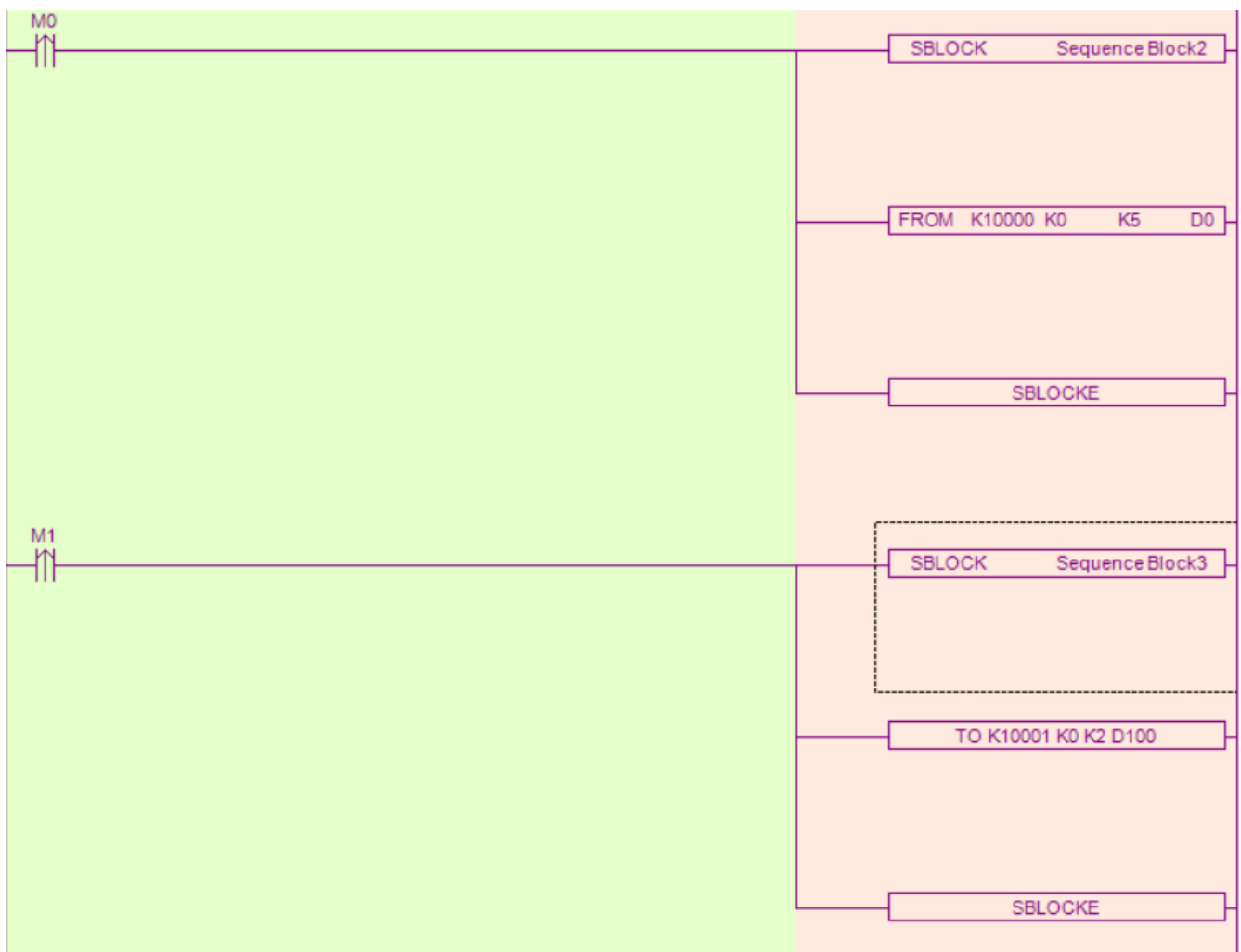
(4) Ladder chart
