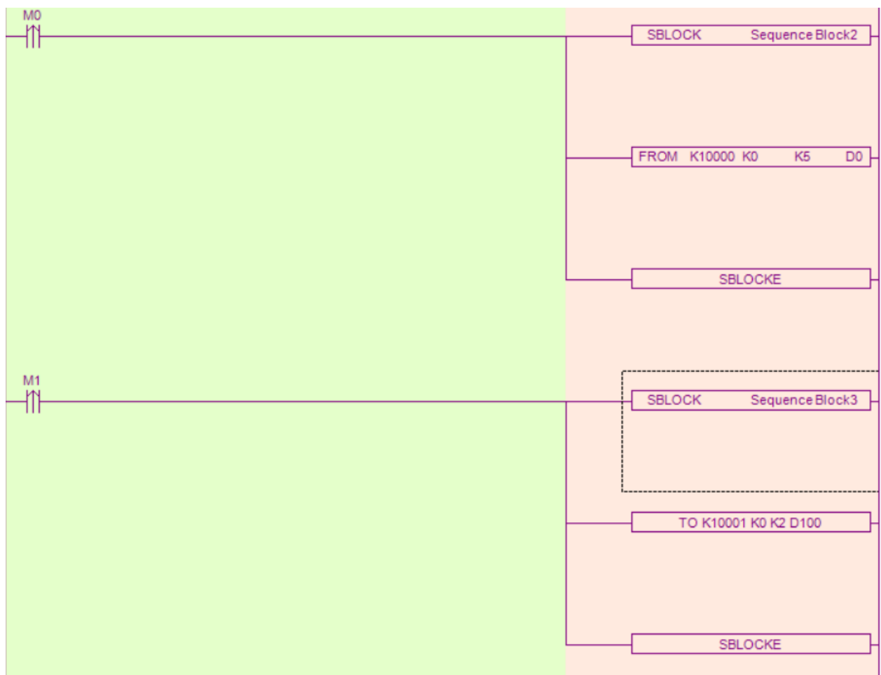
(4) Ladder chart
