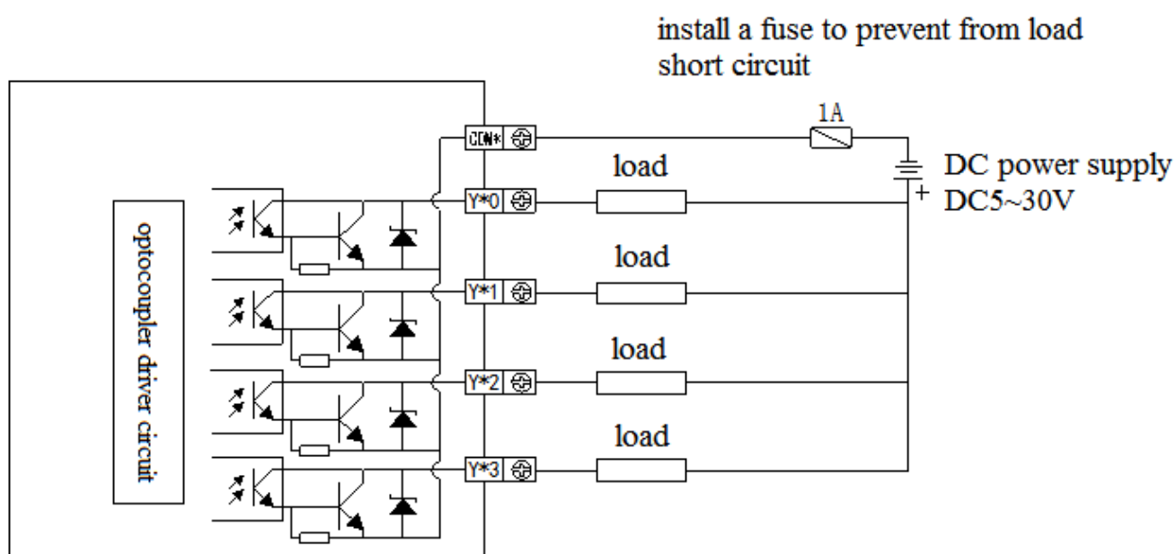
Transistor type
