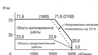
R88M-KH5K020F/C (400 В, 5 кВт)
